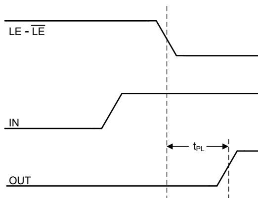
Figure 6-4. Latch Disable with Input Change
