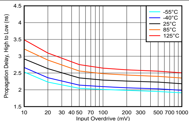
Figure 5-30. Propagation Delay, High to Low, 3.3V
