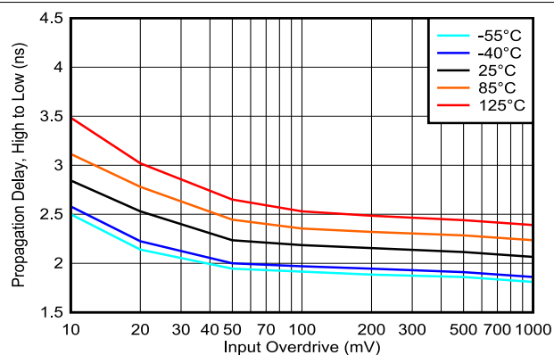
Figure 5-32. Propagation Delay, High to Low, 5V
