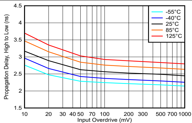
Figure 5-28. Propagation Delay, High to Low, 2.5V
