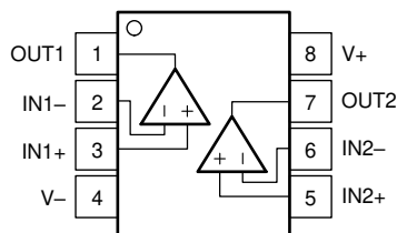
DGK, DSG Packages 8-Pin VSSOP, WSON Top View
