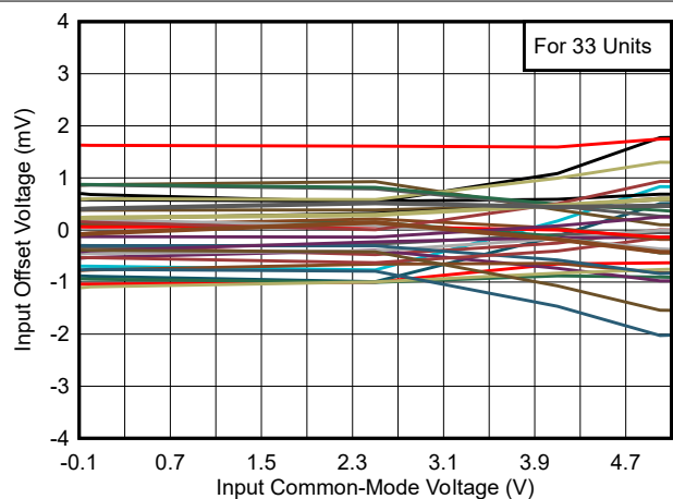
Figure 5-5. Offset vs. Common-Mode, 5V
