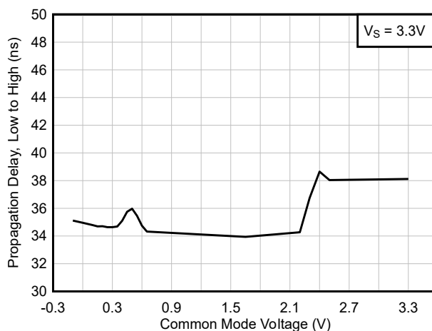
Figure 5-40. Propagation Delay, Low to High vs. Common Mode at 3.3V
