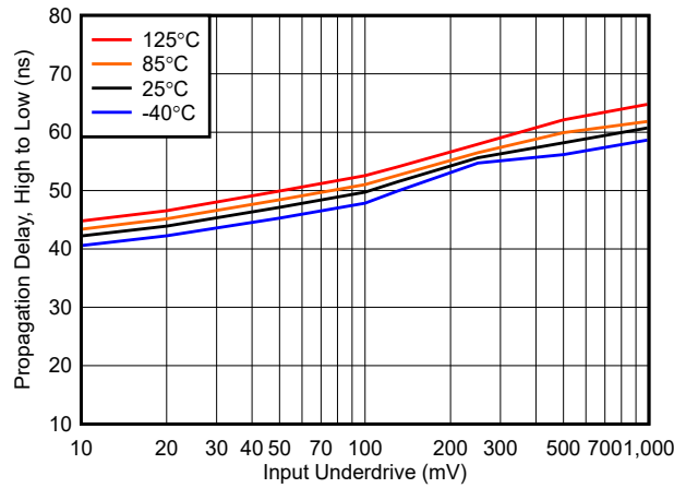
Figure 5-31. Propagation Delay, High to Low vs. Underdrive at 1.8V
