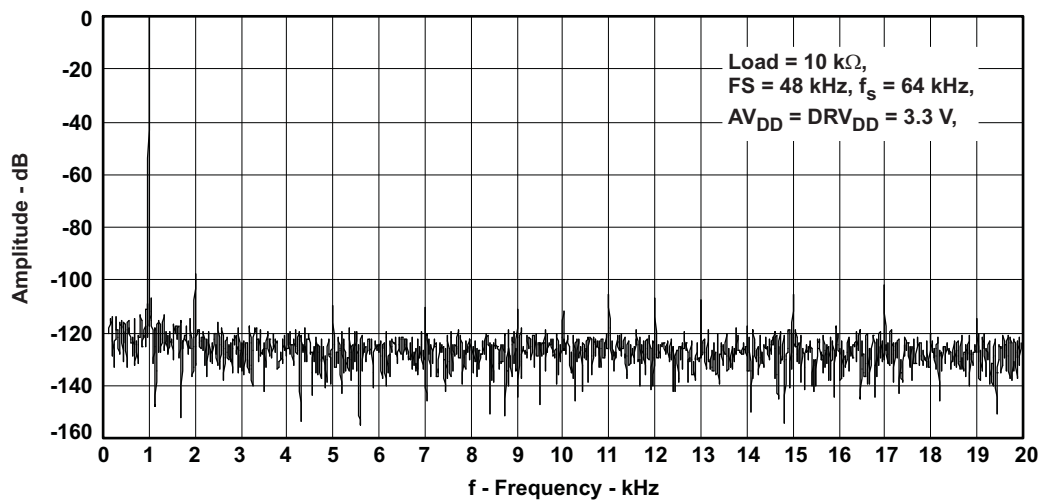
Figure 10. Right-DAC FFT
