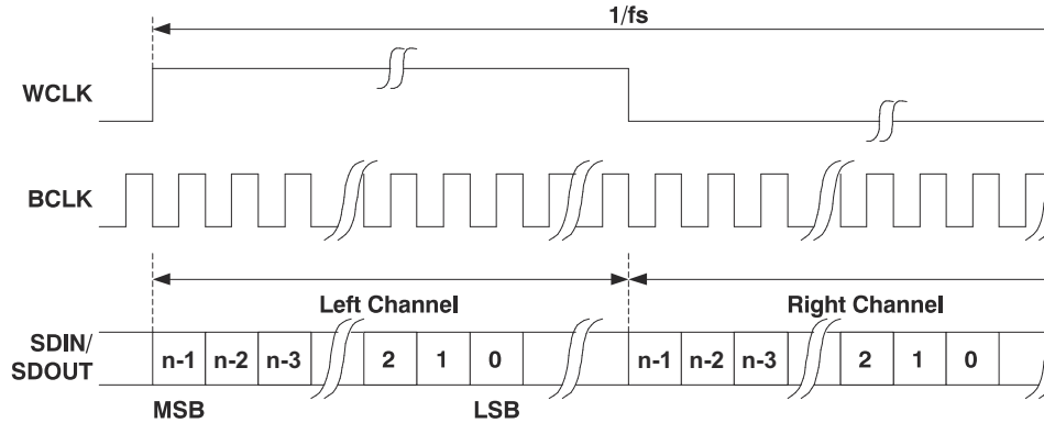
Figure 10-4. Left-Justified Serial Data Bus Mode Operation
