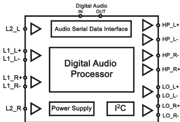
Simplified Diagram
