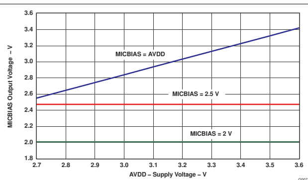
Figure 11-3. MICBIAS Output Voltage vs AVDD
