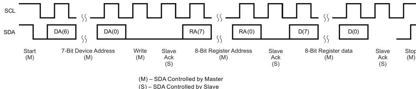
Figure 10-24. I²C Write
