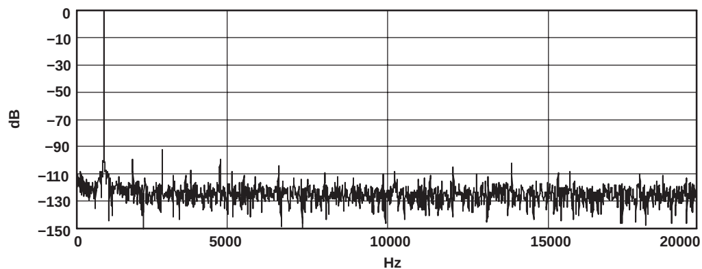
Figure 11. DAC FFT Plot ( T_A = 25^\circ\text{C} , 48 kpsps, -1 dB, 1 kHz Input, AVDD = DRVDD = 3.3\text{ V} , DVDD = 1.8\text{ V} , R_L = 16\ \Omega )
