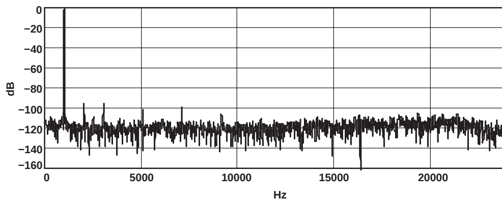
Figure 8. ADC FFT Plot at 48 ksps ( T_A = 25^\circ\text{C} , -1\text{ dB} , 1\text{ kHz} Input, \text{AVDD} = 3.3\text{ V} )
