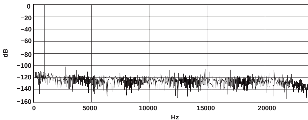
Figure 10. DAC FFT Plot ( T_A = 25^\circ\text{C} , 48\text{ ksps} , 0\text{ dB} , 1\text{ kHz} Input, \text{AVDD} = 3.3\text{ V} , R_L = 10\text{ k}\Omega )
