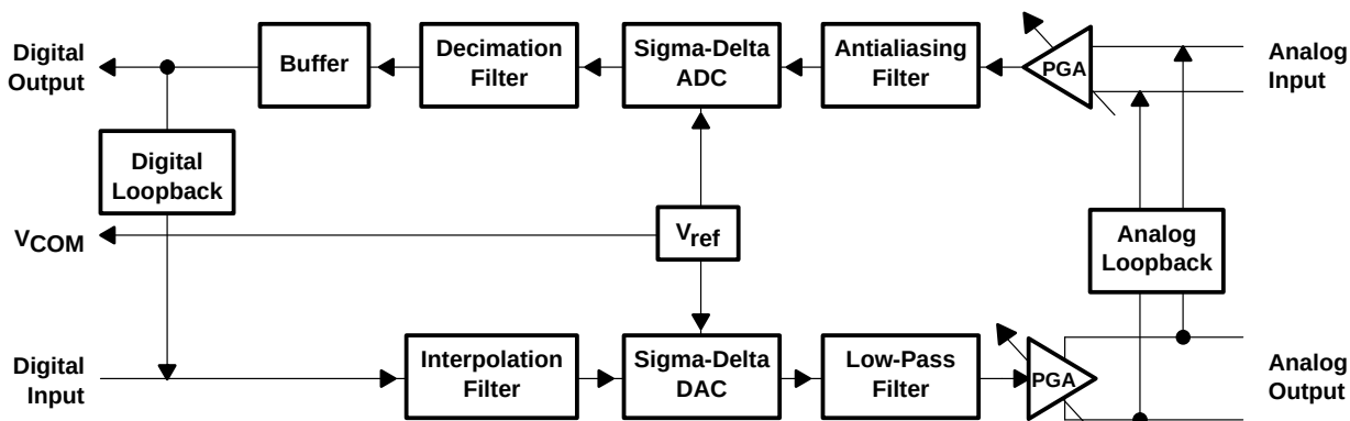
functional block diagram (one of two codecs shown)
