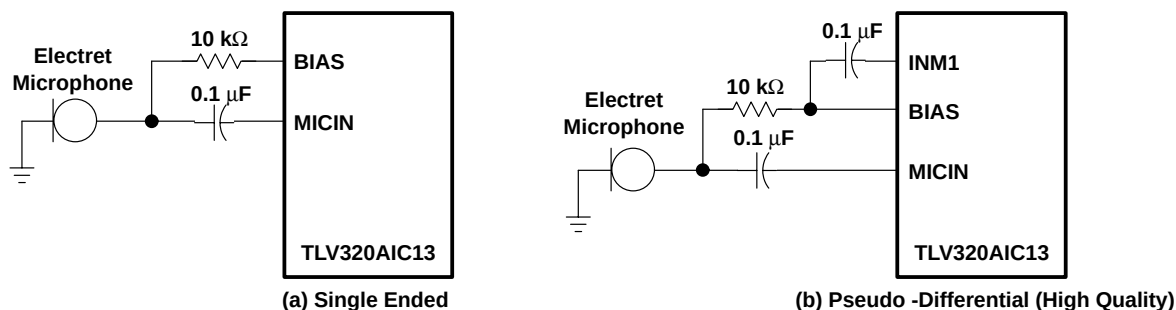
Figure 3–1. Microphone Interface
