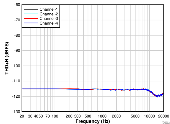
Figure 7-25. PDM Input THD+N vs Input Frequency With a -20-dBr Input
