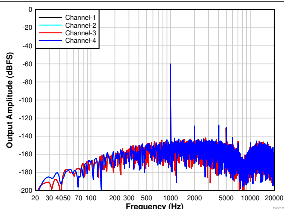
Figure 7-26. PDM Input FFT With a -60-dBr Input
