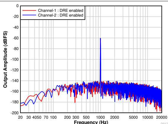
Figure 7-20. FFT With a -60-dBr Input With DRE Enabled
