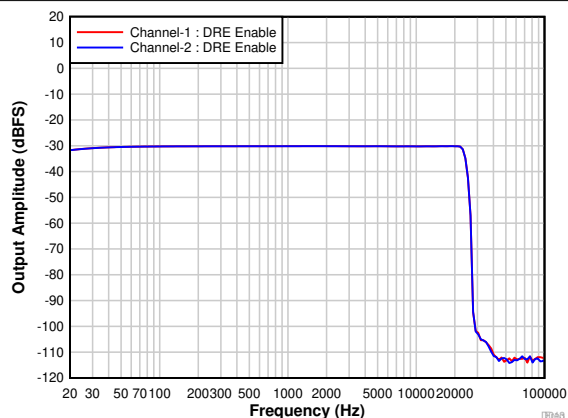
Figure 7-16. Frequency Response With a -30-dBr Input
