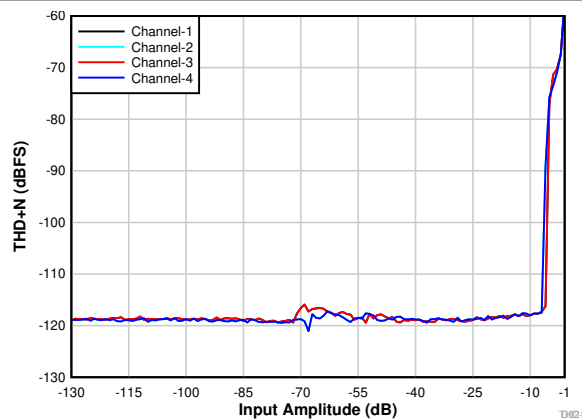
Figure 7-24. PDM Input THD+N vs Input Amplitude
