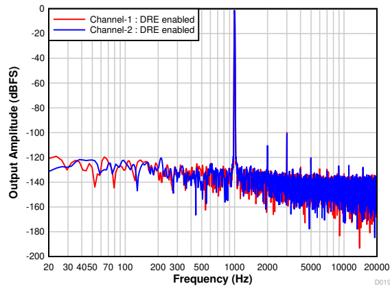
Figure 7-22. FFT With a -1-dBr Input With DRE Enabled
