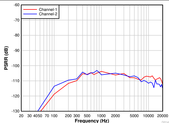
Figure 7-17. Power-Supply Rejection Ratio vs Ripple Frequency With 100-mV pp Amplitude
