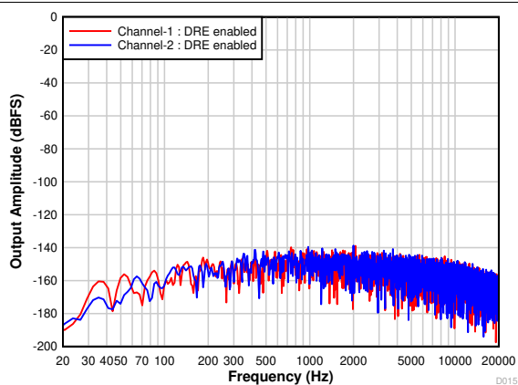
Figure 7-18. FFT With Idle Input With DRE Enabled
