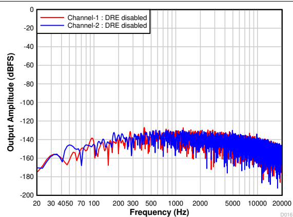
Figure 7-19. FFT With Idle Input With DRE Disabled
