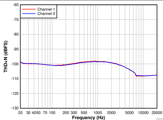
Figure 7-10. THD+N vs Input Frequency With a -60\text{-dBr} Input
