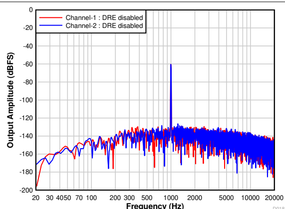
Figure 7-21. FFT With a -60-dBr Input With DRE Disabled
