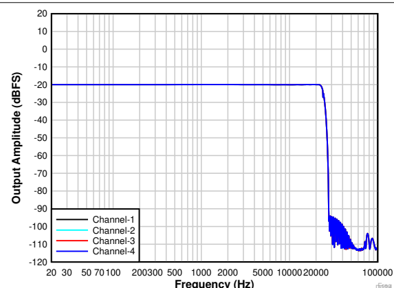
Figure 7-27. PDM Input Frequency Response With a -20-dBr Input
