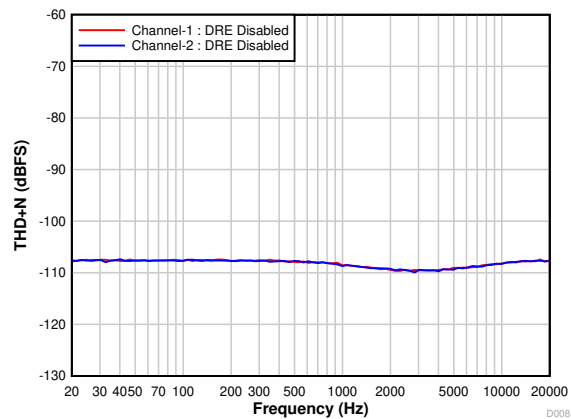
Figure 7-11. THD+N vs Input Frequency With a -60\text{-dBr} Input
