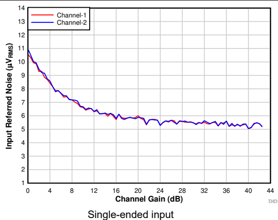
Figure 7-14. Input-Referred Noise vs Channel Gain
