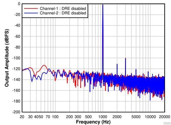
Figure 7-23. FFT With a -1-dBr Input With DRE Disabled
