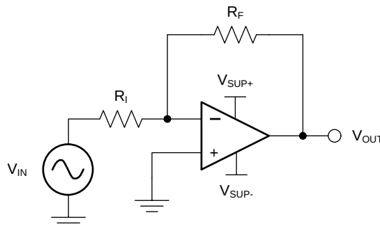
Figure 15. Application Schematic
