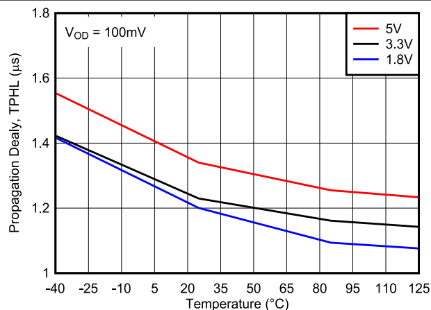
Figure 6-14. High to Low Propagation Delay vs. Temperature
