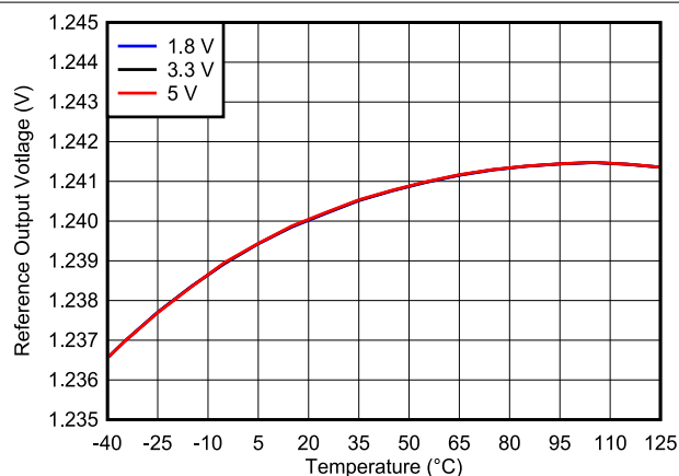
Figure 6-16. Reference Voltage vs. Temperature
