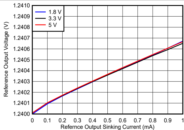
Figure 6-18. Reference Voltage vs. Reference Output Sinking Current
