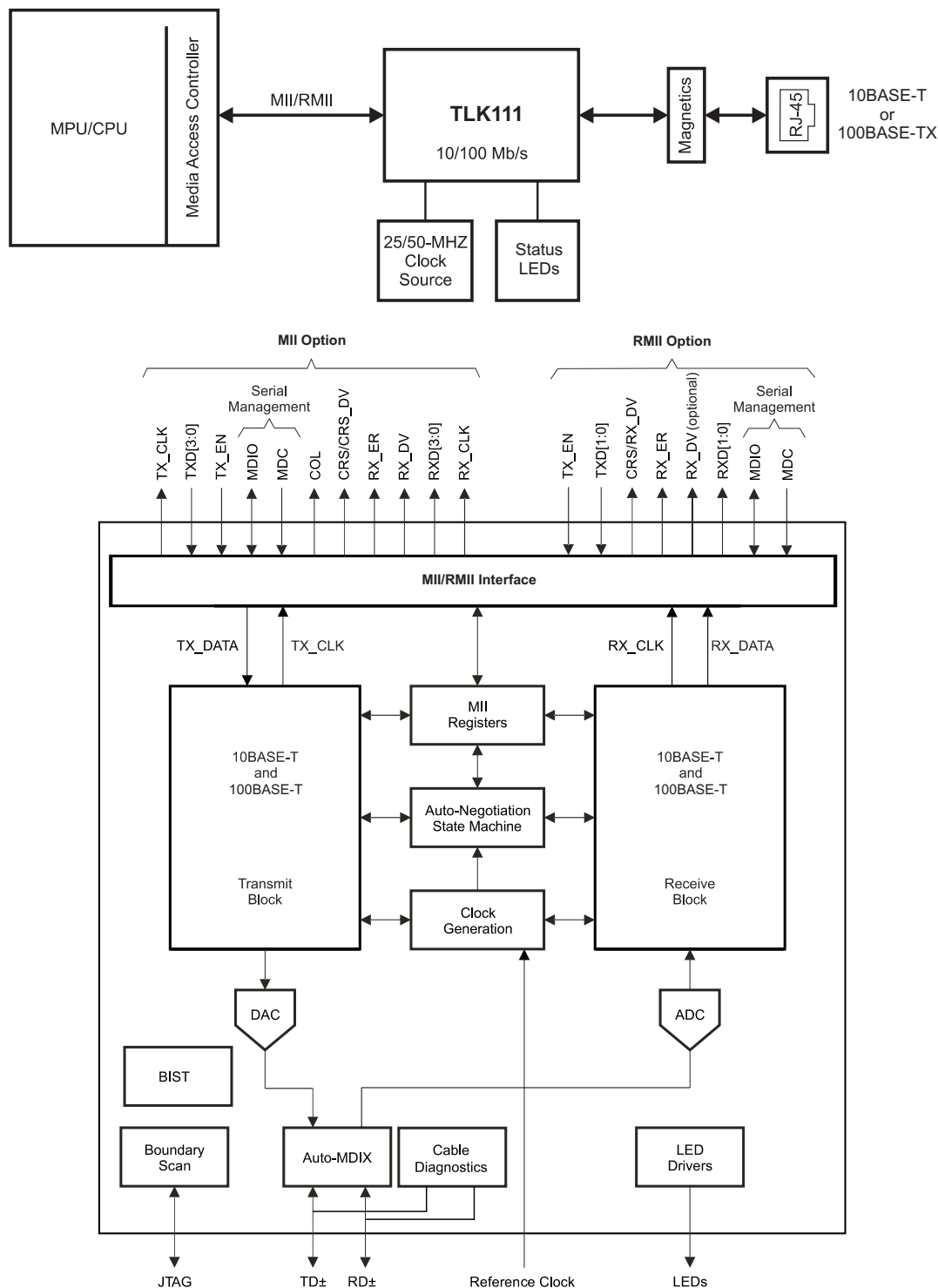
Figure 1-1. TLK111 Functional Block Diagram
