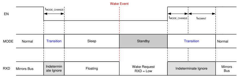
Figure 6-5. Mode Transitions
