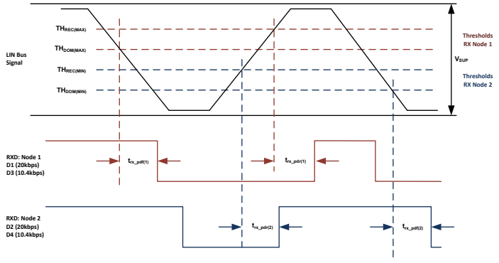
Figure 6-4. Propagation Delay
