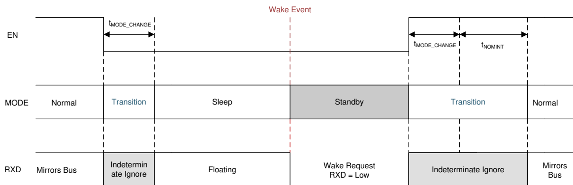
Figure 8-14. Mode Transitions
