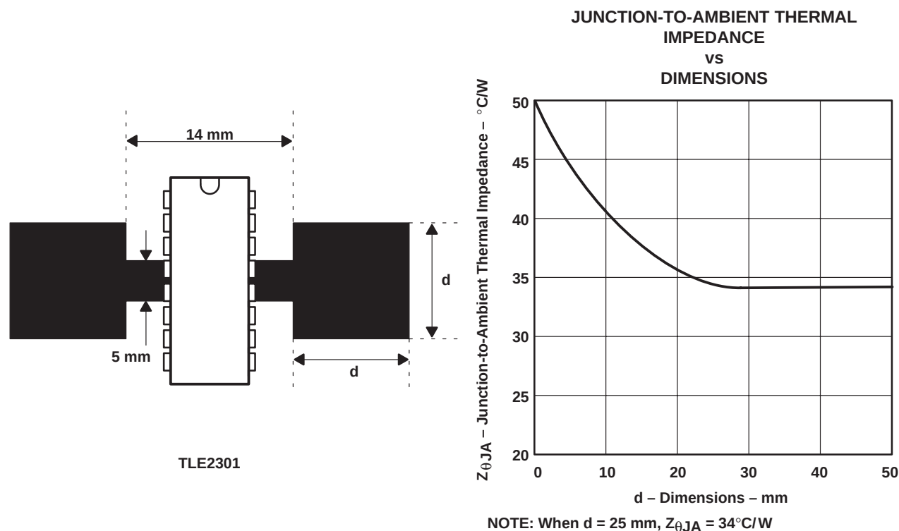
Figure 27. PCB Heatsink
