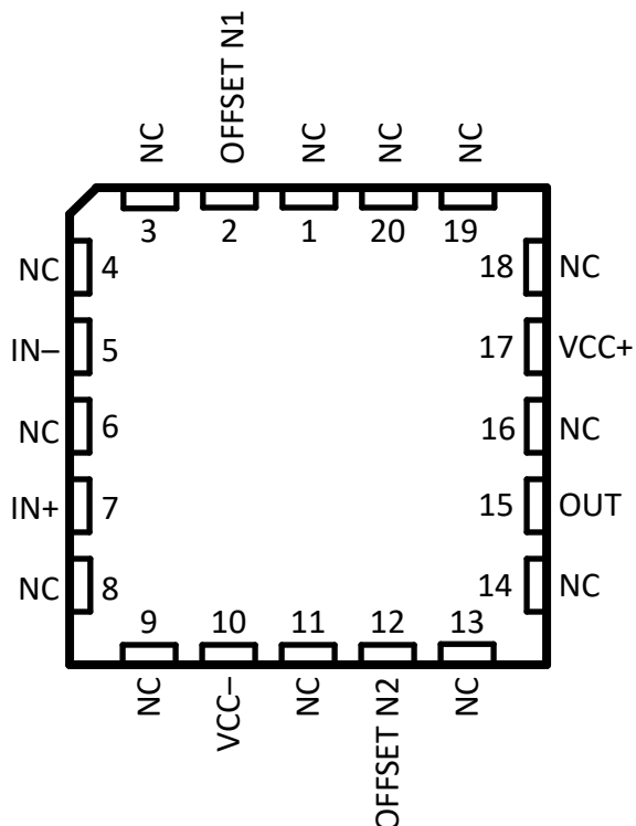
Figure 5-6. TLE2071M and TLE2071AM FK PACKAGE (Top View)
