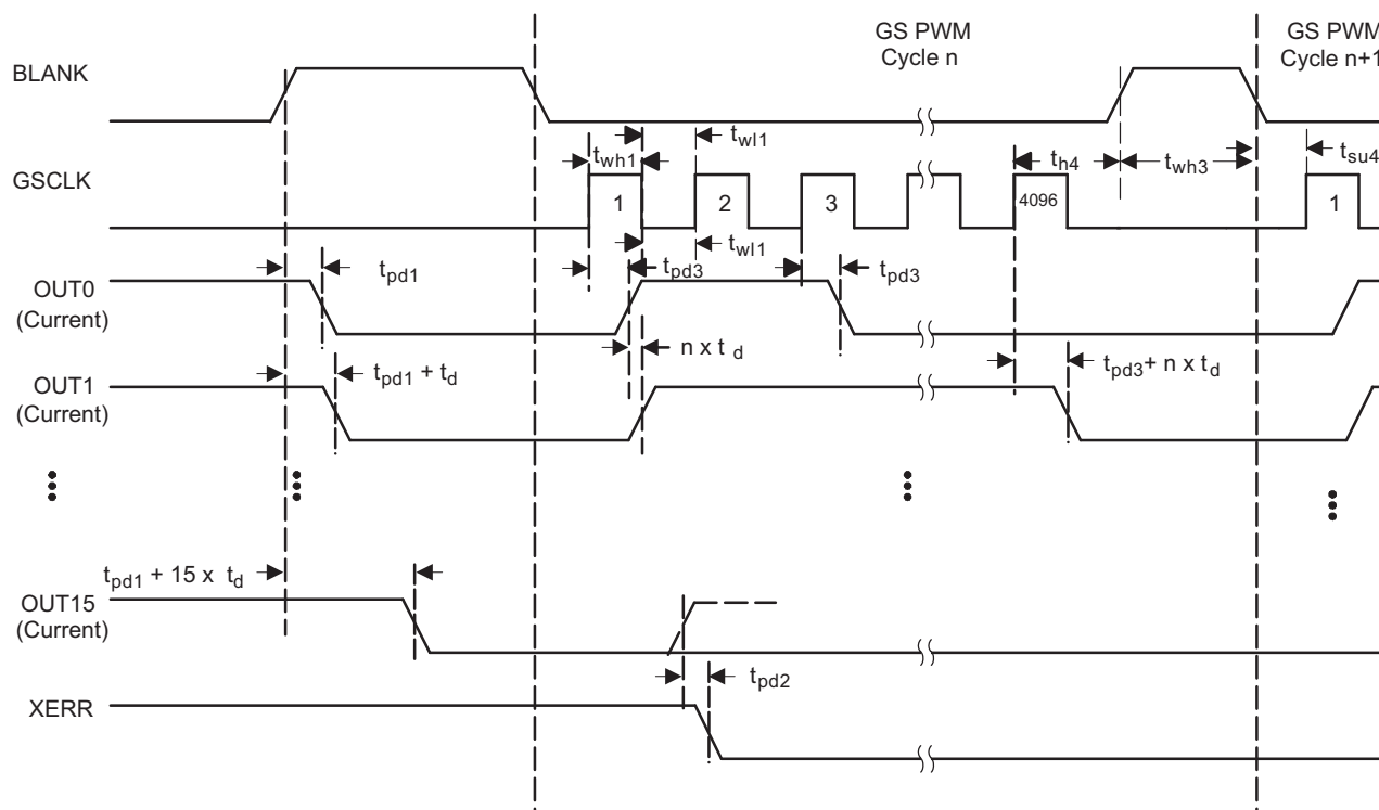
Figure 17. Grayscale PWM Cycle Timing Chart
