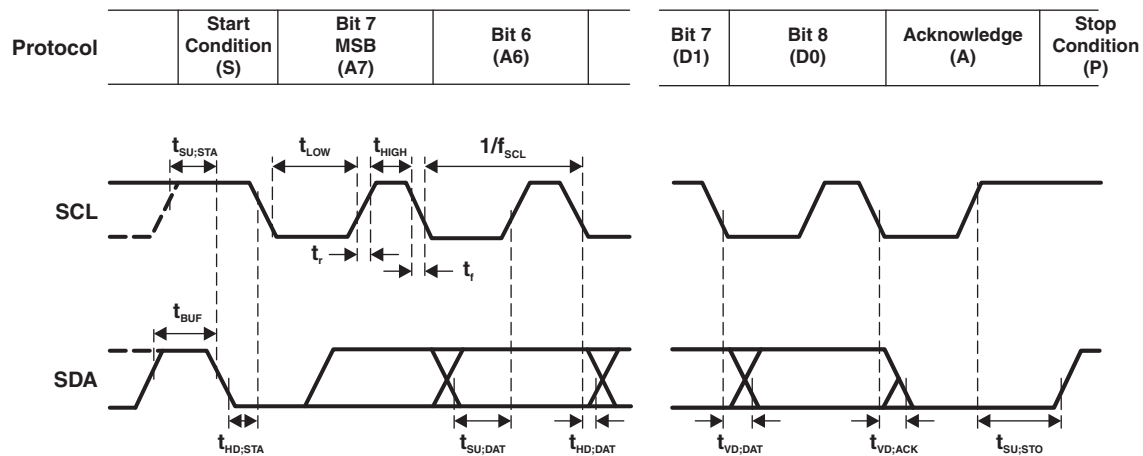
Figure 5. I²C Bus Timing
