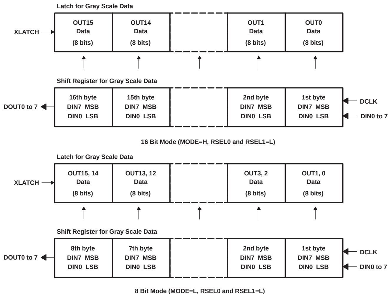
Figure 3. Relationship Between Shift Register and Latch for Gray Scale Data
