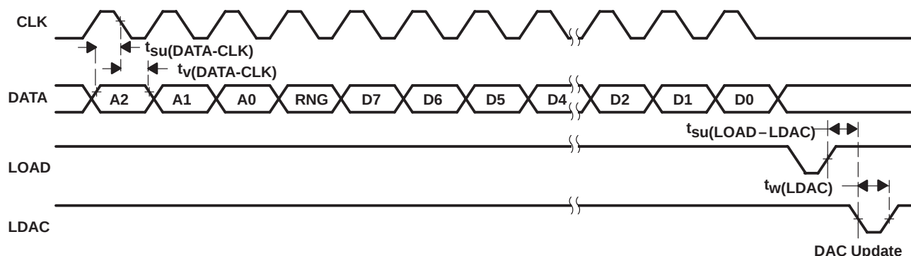
Figure 2. LDAC-Controlled Update
