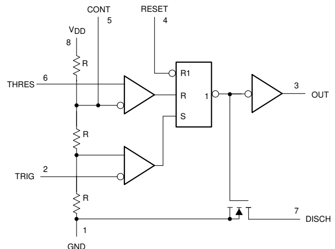
Simplified Schematic
