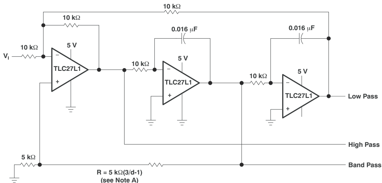
Figure 7-10. State-Variable Filter
