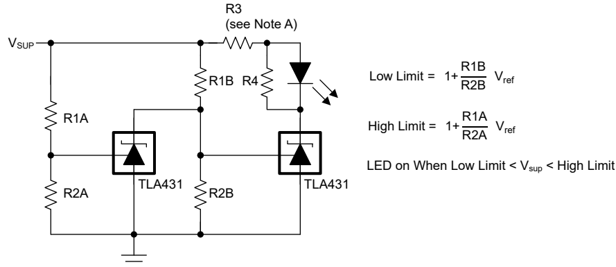
Figure 9-8. Voltage Monitor
