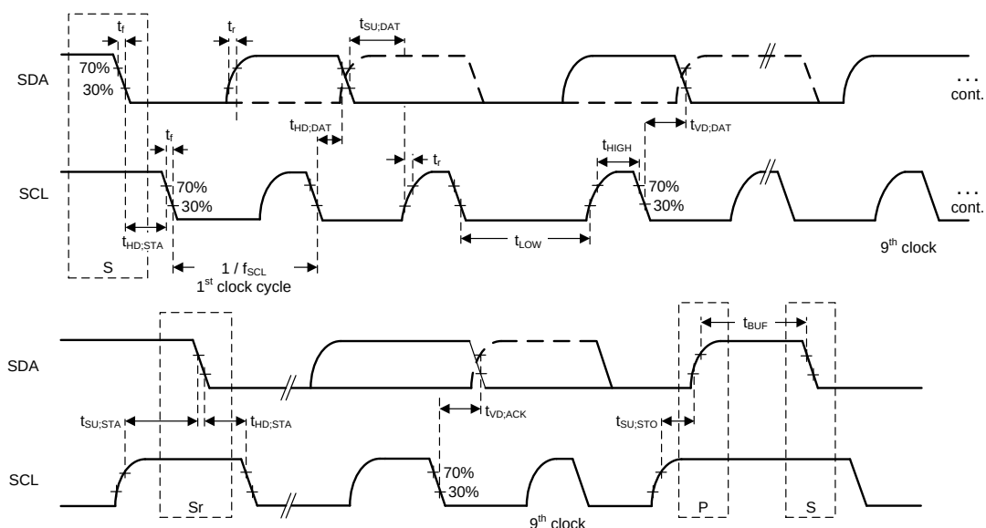
Figure 1. I 2 C Timing Requirements
