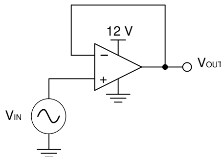
Figure 7-1. Voltage Follower Schematic
