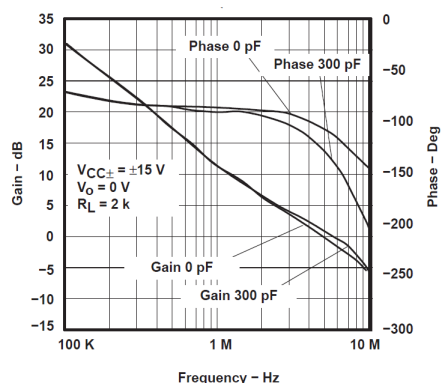
Figure 5-3. Gain and Phase vs Frequency, Old Die
