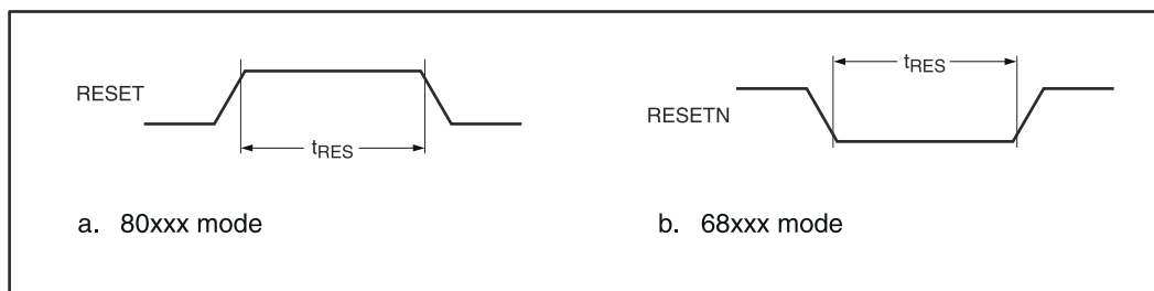
Figure 4-2. Reset Timing
