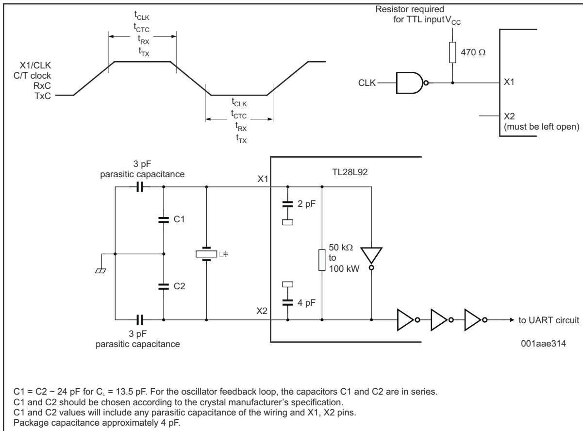
Figure 4-9. Clock Timing
