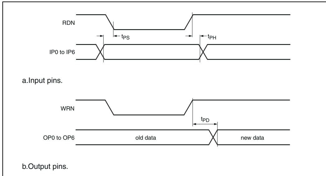
Figure 4-7. Port Timing
