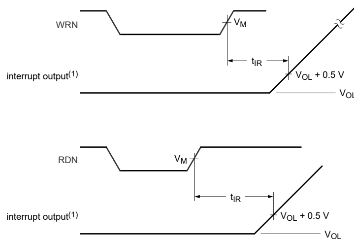
Figure 4-7. Port Timing
