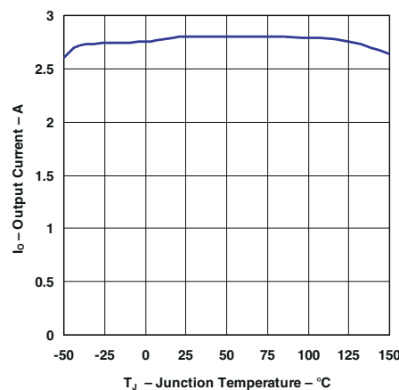
Figure 6-4. Current Limit
