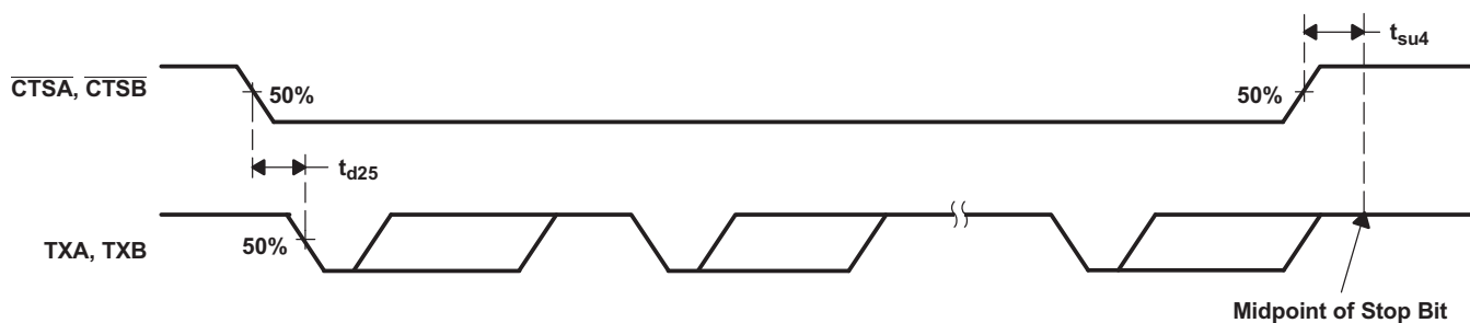
Figure 22. CTS and TX Autoflow Control Timing (Start and Stop) Waveforms
