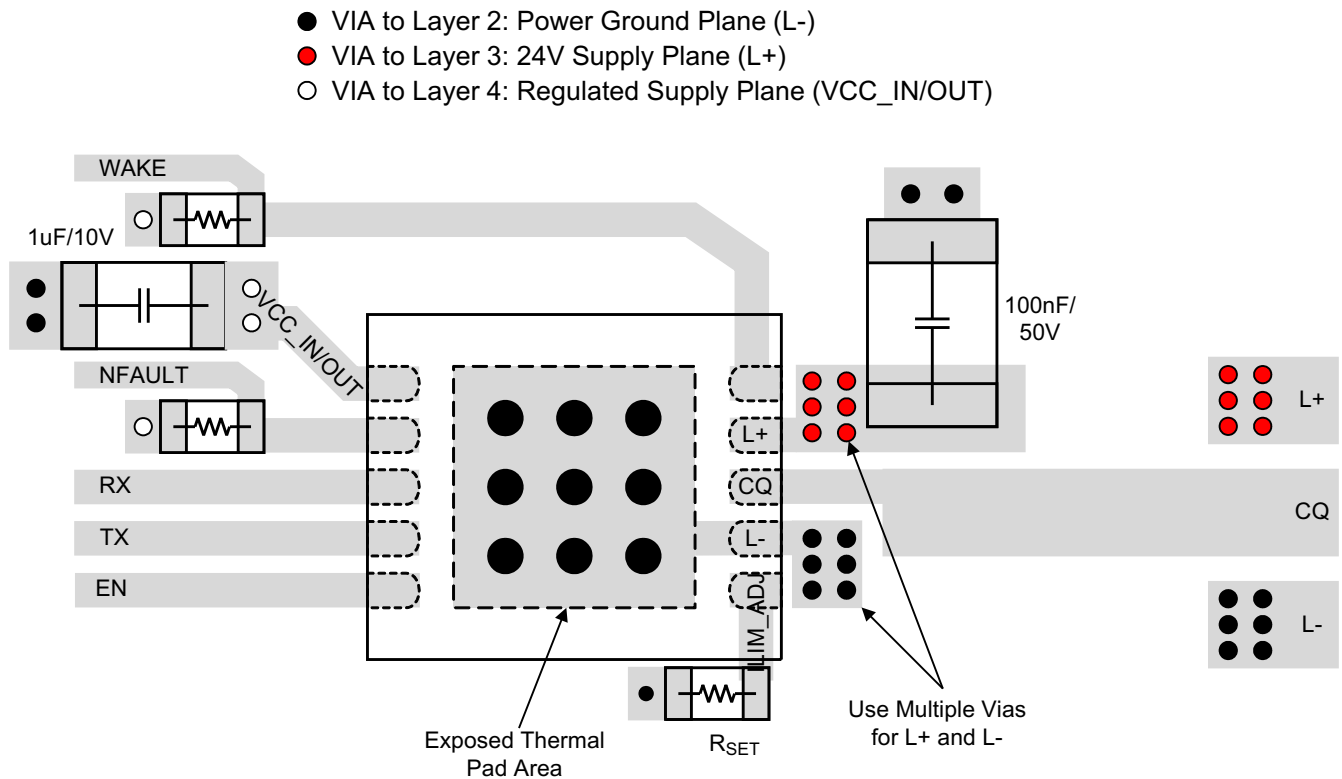
Figure 9-9. Layout Example
