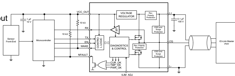
Typical Application Diagram
