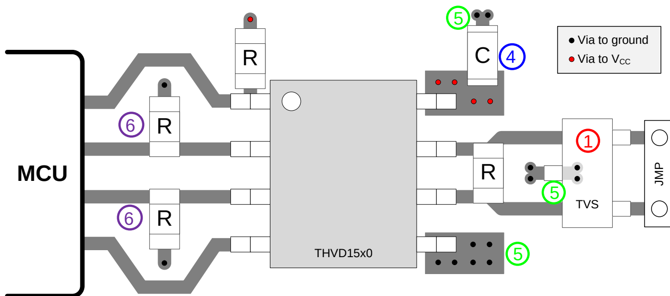
Figure 32. Half-Duplex Layout Example
