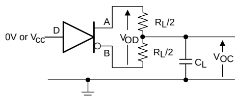
Figure 12. Measurement of Driver Differential and Common-Mode Output With RS-485 Load
