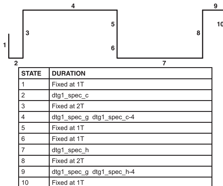
Figure 6-32. SDTV Line Type NEQ_BSP
