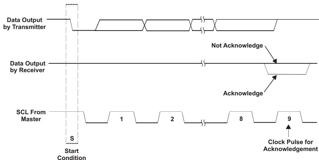
Figure 73. I²C Acknowledge
