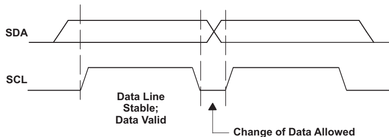
Figure 72. I²C Bit Transfer
