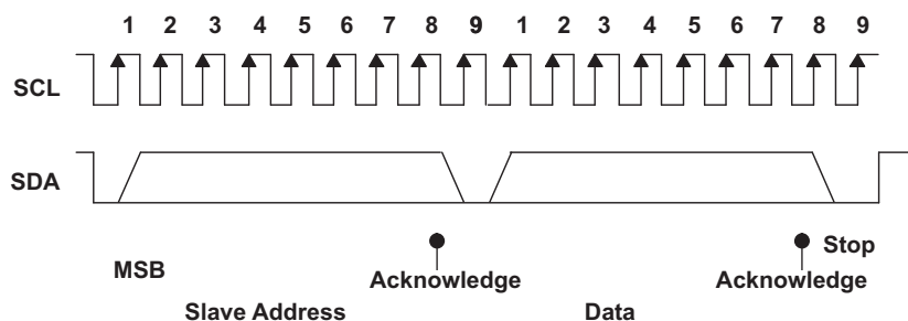
Figure 74. I²C Address and Data Cycles
