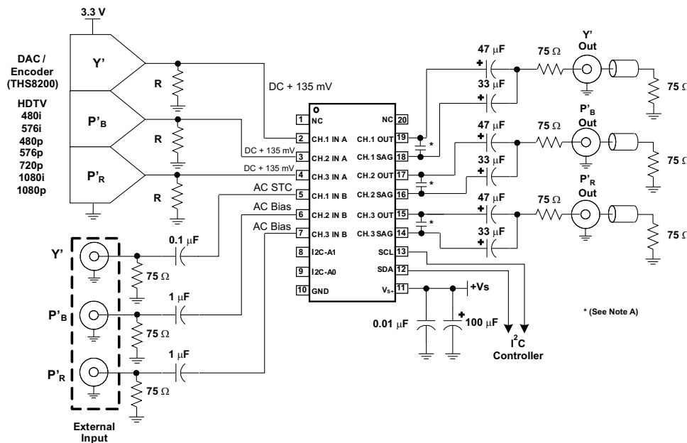
Figure 67. Typical Y'P R P R System Driving SAG Corrected AC-Coupled Video Lines
