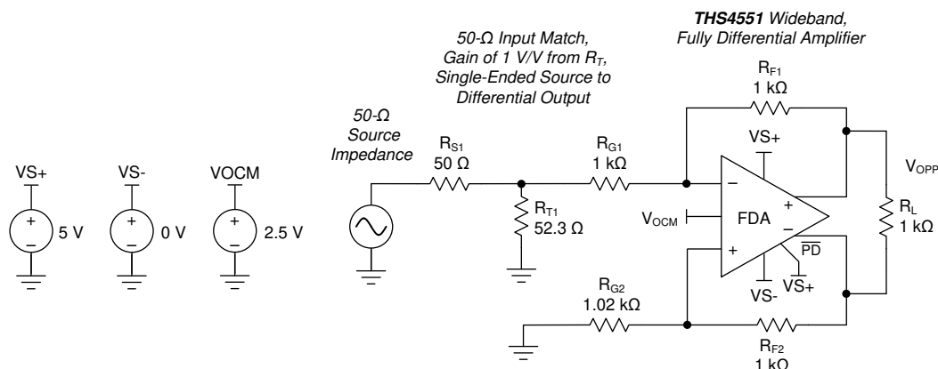
Figure 9-9. DC-Coupled Gain of 1 with R_F = 1 kΩ and Single-to-Differential Matched Input 50-Ω Impedance
