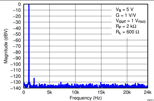
Figure 81. 1-kHz FFT Plot on Audio Analyzer
