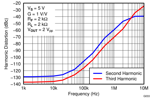
Figure 41. Harmonic Distortion vs Frequency
