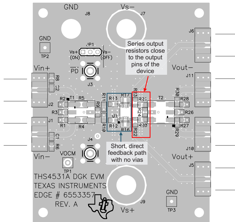
Figure 98. THS4531ADGKEVM Top Layer 1
