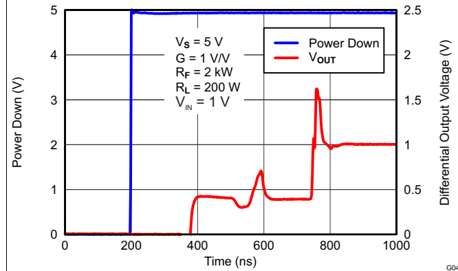
Figure 53. Turnon Time
