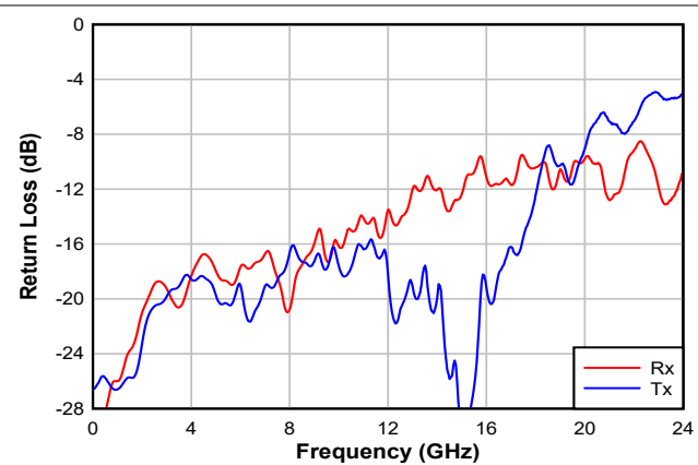
Figure 5-2. Typical Differential Return Loss
