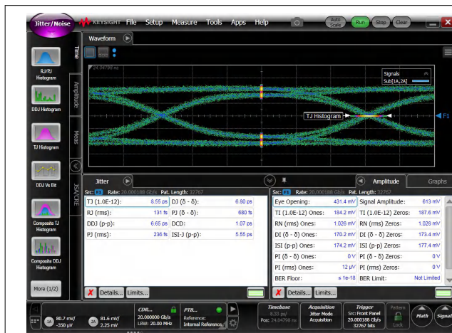
Figure 5-3. Through Baseline Calibration Trace Setup for 20Gbps
