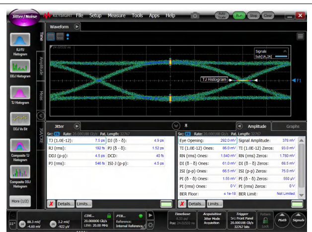
Figure 5-4. Through TDP2044 for 20Gbps
