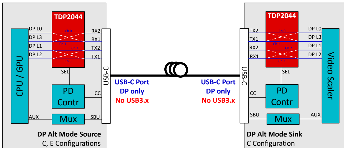
Figure 7-1. Typical Application
