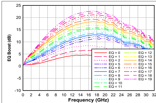
Figure 5-1. Typical EQ Boost vs Frequency
