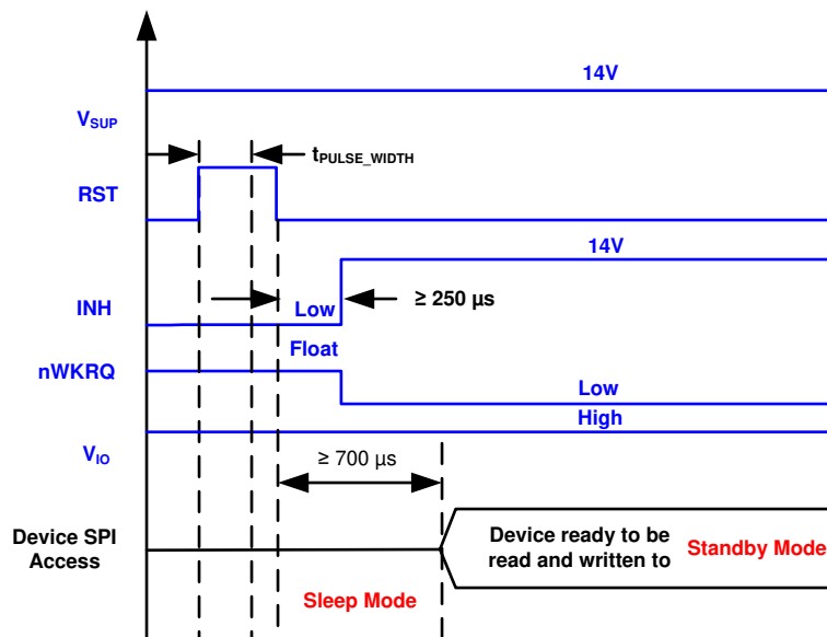
Figure 8-4. Timing for RST Pin in Sleep Mode
