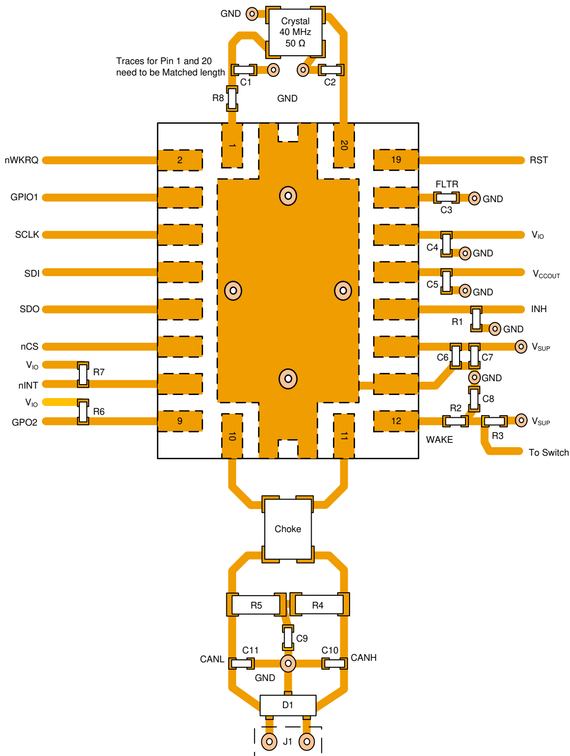
Figure 11-1. Example Layout
