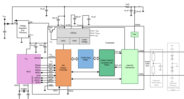
Simplified Schematics, CLKIN from MCU
