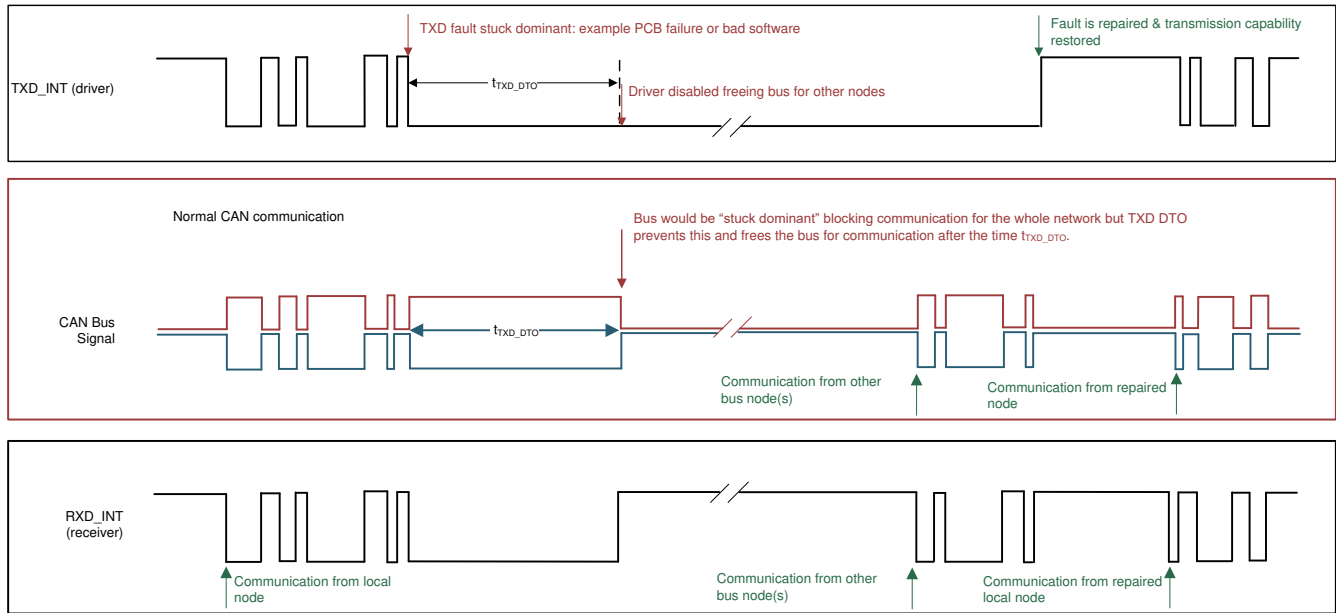
Figure 8-7. Example timing diagram with TXD_INT DTO
