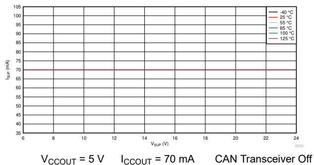
Figure 6-2. I_{SUP} Current Across Temperature and V_{SUP} LDO Output Only.
