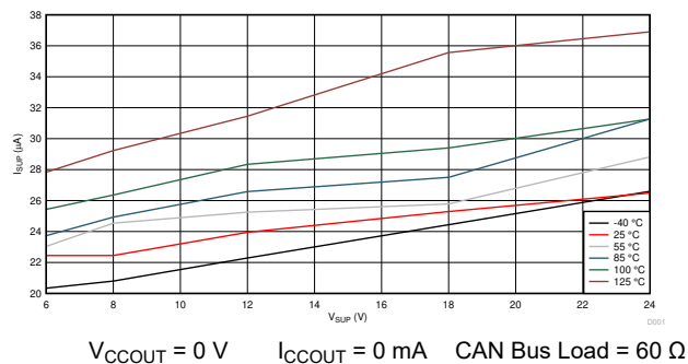
Figure 6-1. I_{SUP} vs V_{SUP} Sleep Mode
