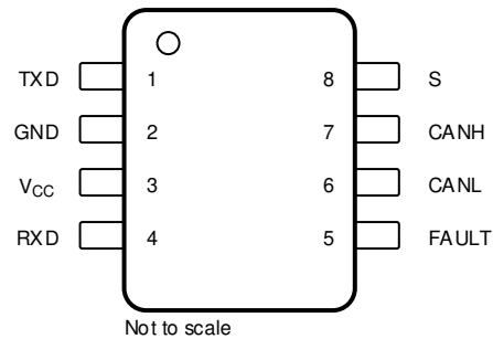
Figure 4-4. TCAN337 D, DCN Packages, 8-Pin SOIC, SOT-23, (Top View)
