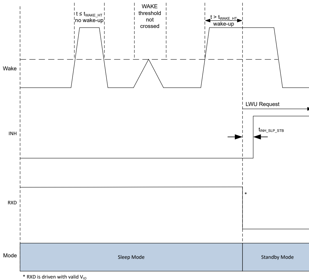
Figure 9-10. LWU Request Rising Edge
