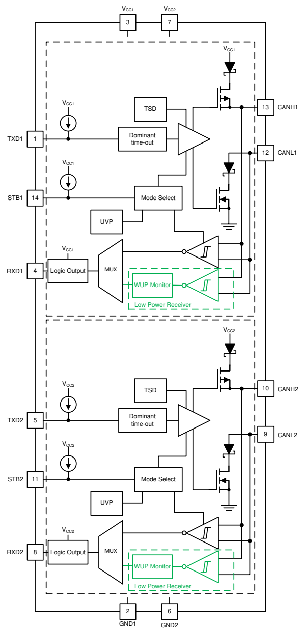
Figure 8-1. Block Diagram
