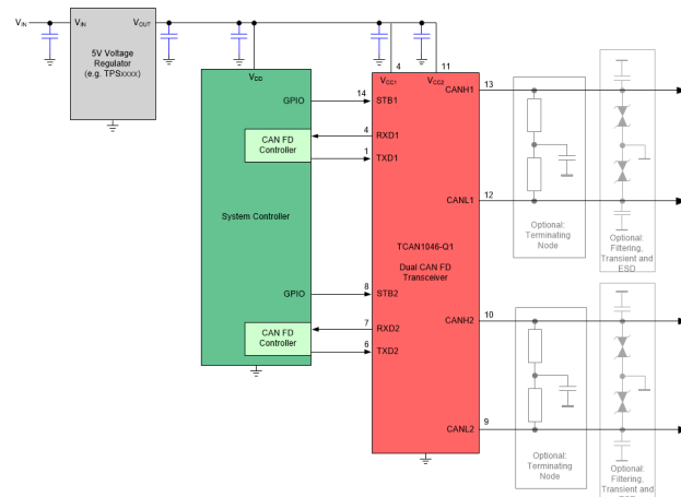
Simplified Schematic
