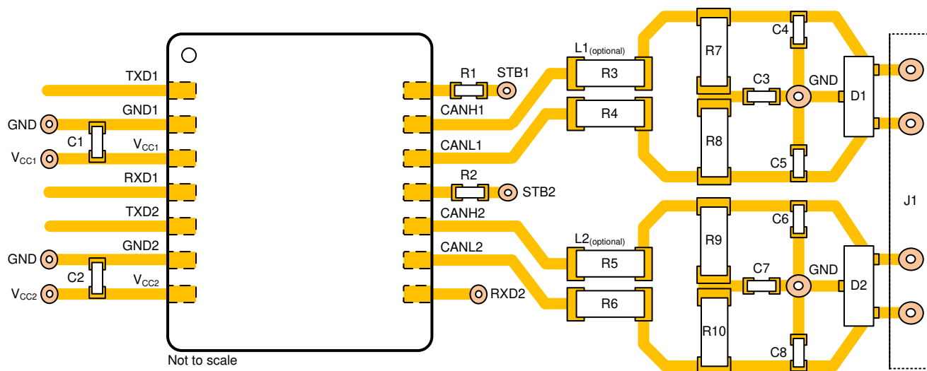
Figure 11-1. Layout Example
