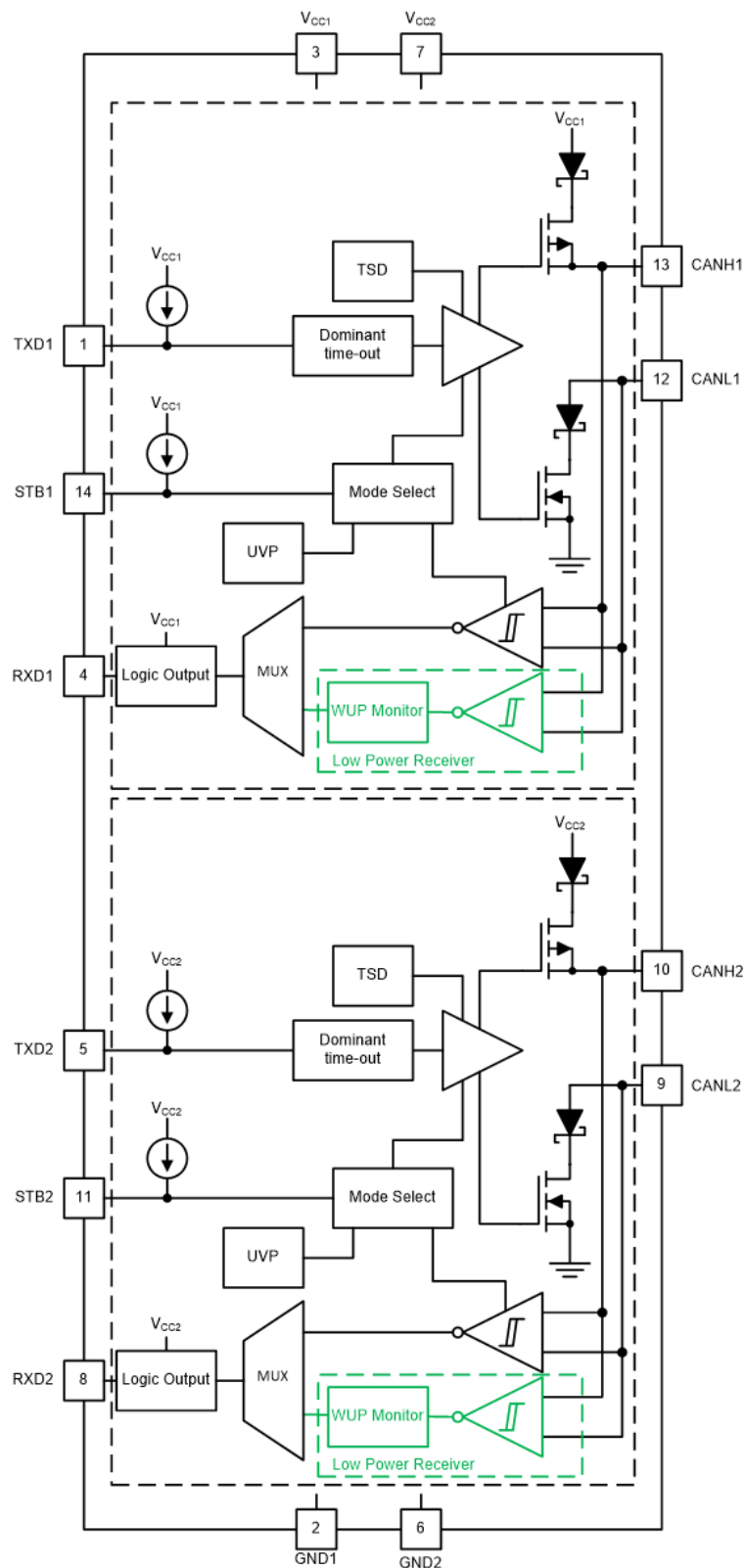
Figure 8-1. Block Diagram
