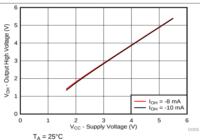
Figure 8. Output High Voltage ( V_{OH} ) vs Supply Voltage ( V_{CC} ) for P-Ports
