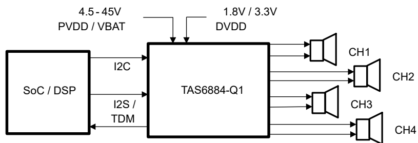
Simplified Diagram
