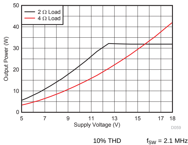
Figure 7. Output Power vs Supply Voltage
