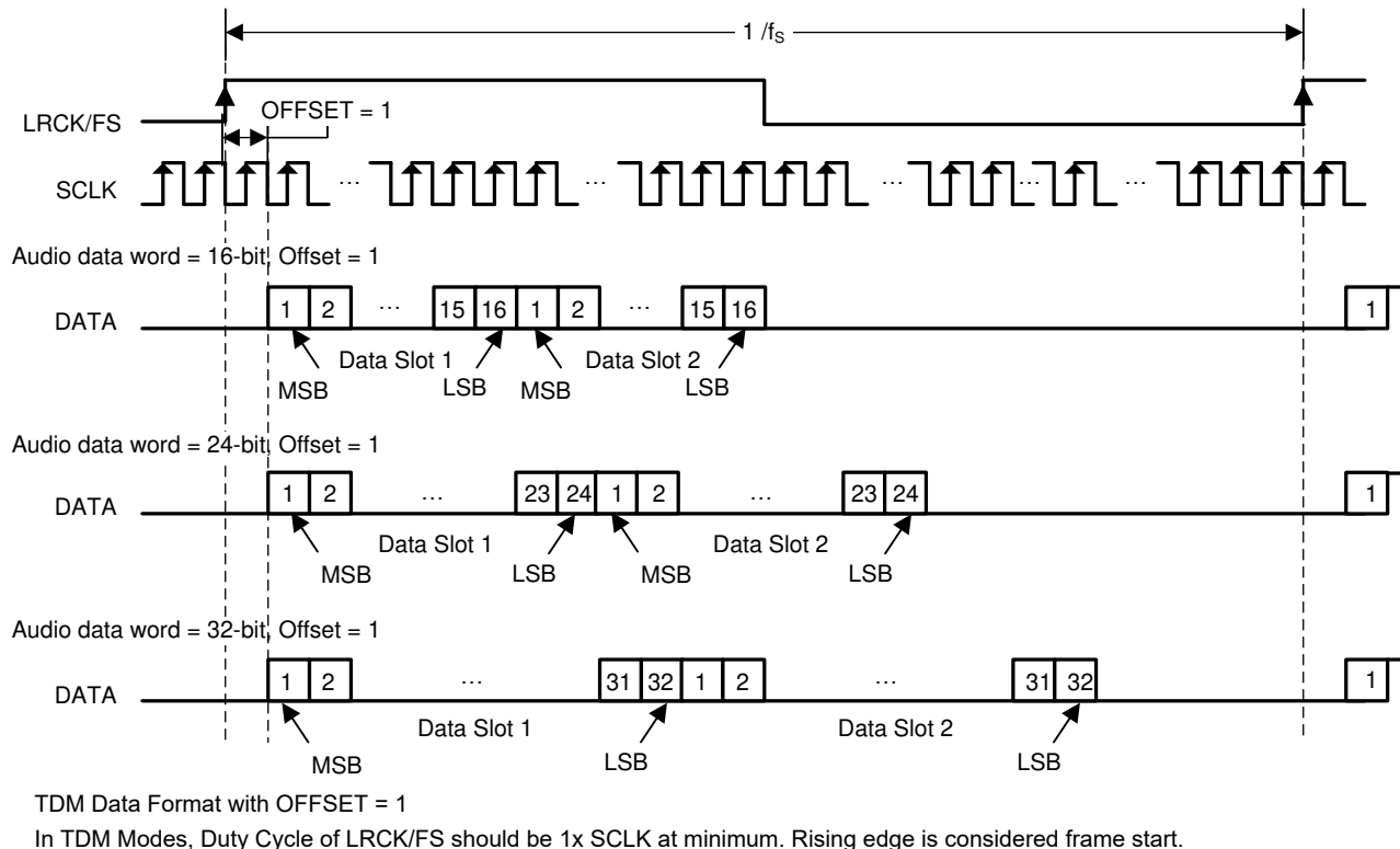
Figure 6-6. TDM 2 Audio Data Format
