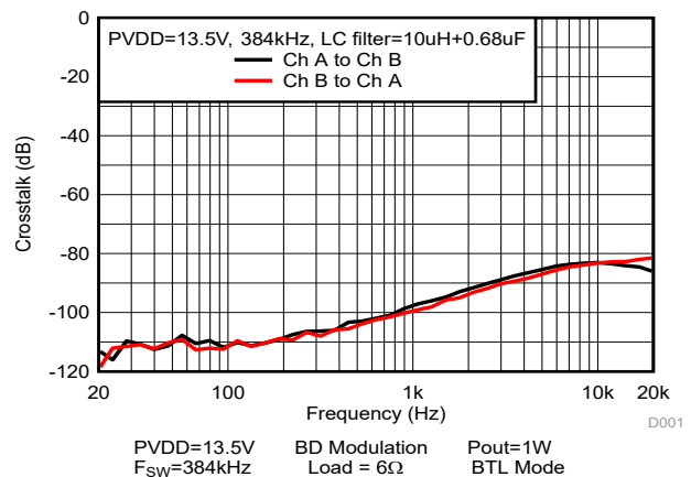
Figure 5-36. Crosstalk
