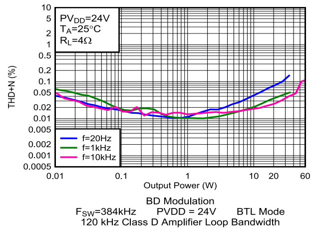
Figure 5-18. THD+N vs Output Power
