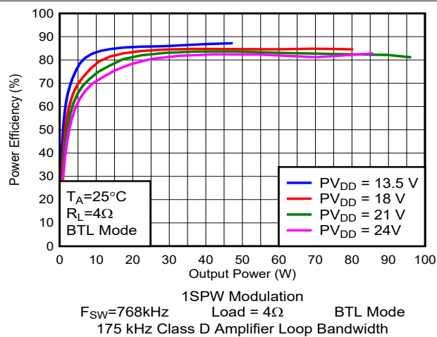
Figure 5-82. Efficiency vs Output Power
