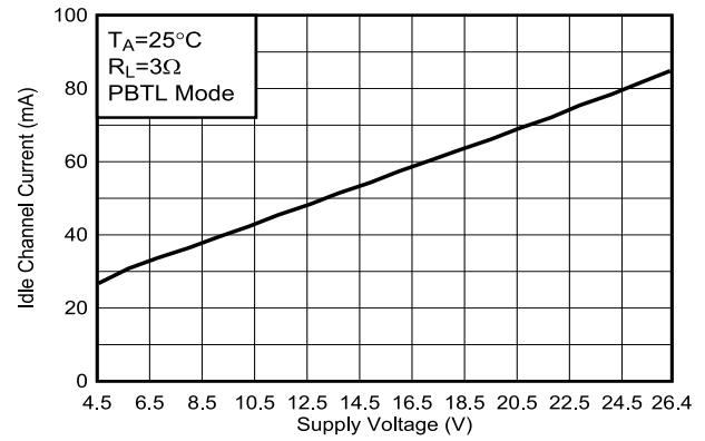
Figure 5-109. PVDD Idle Current vs PVDD Voltage
