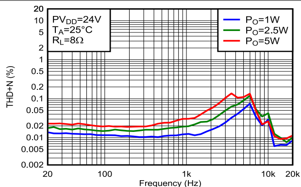
Figure 5-55. THD+N vs Frequency
