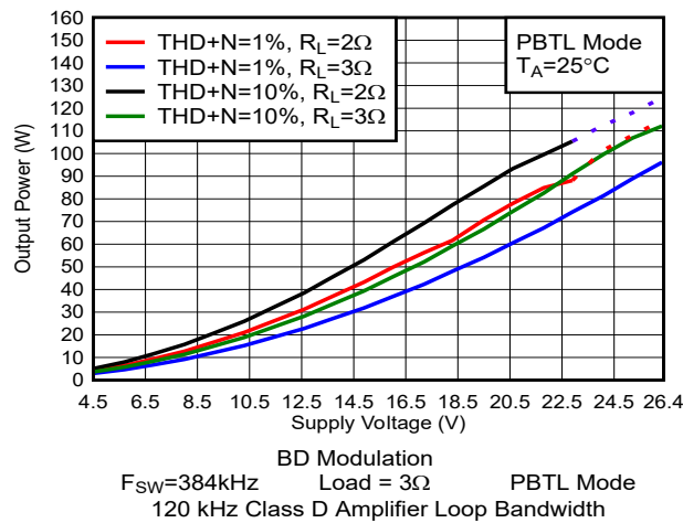
Figure 5-93. Output Power vs Supply Voltage (dotted line is thermally limited)
