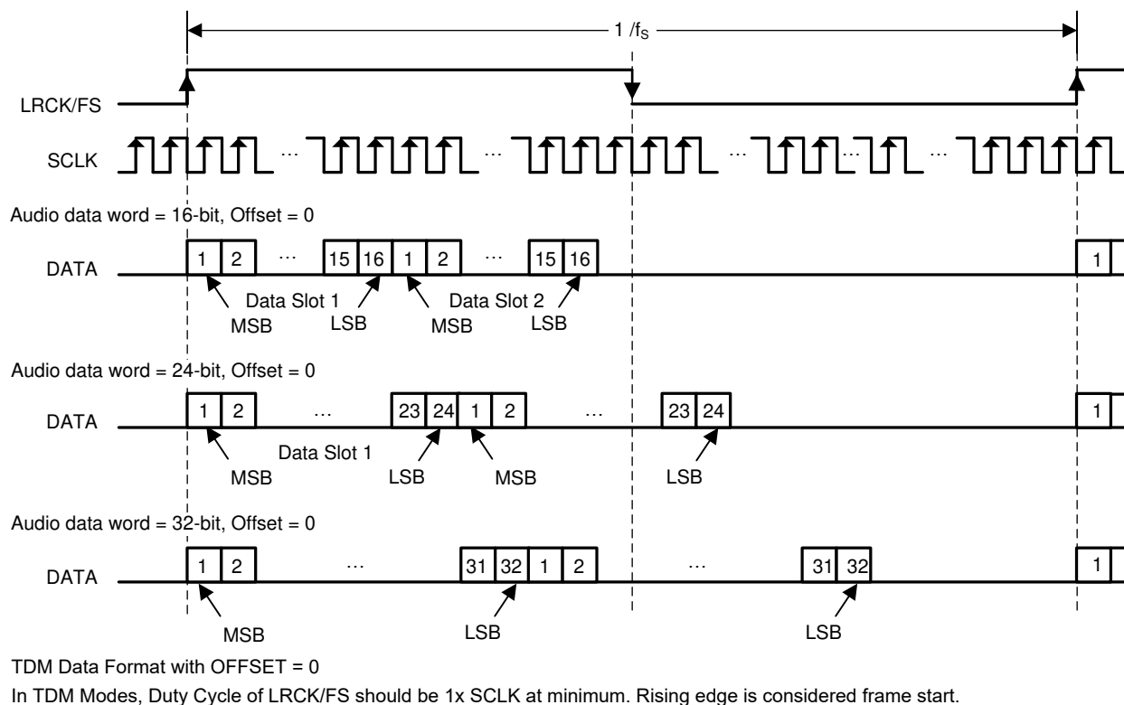
Figure 6-5. TDM 1 Audio Data Format
