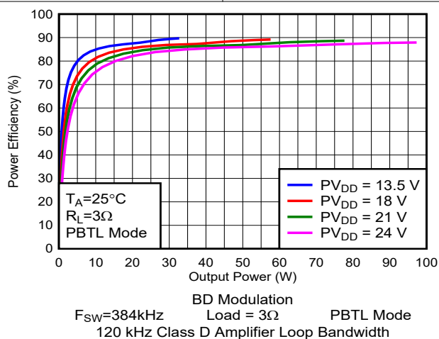
Figure 5-97. Efficiency vs Output Power
