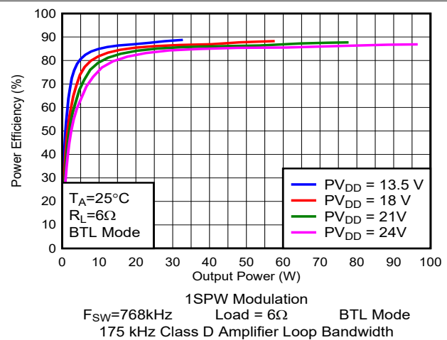
Figure 5-83. Efficiency vs Output Power
