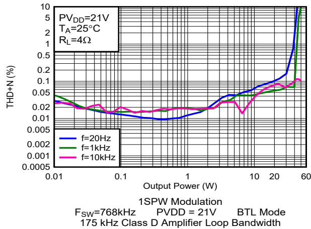
Figure 5-60. THD+N vs Output Power
