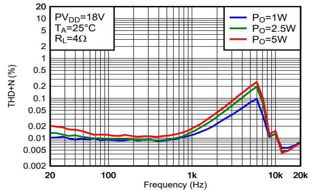
Figure 5-2. THD+N vs Frequency
