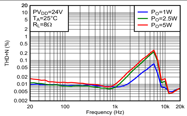
Figure 5-10. THD+N vs Frequency
