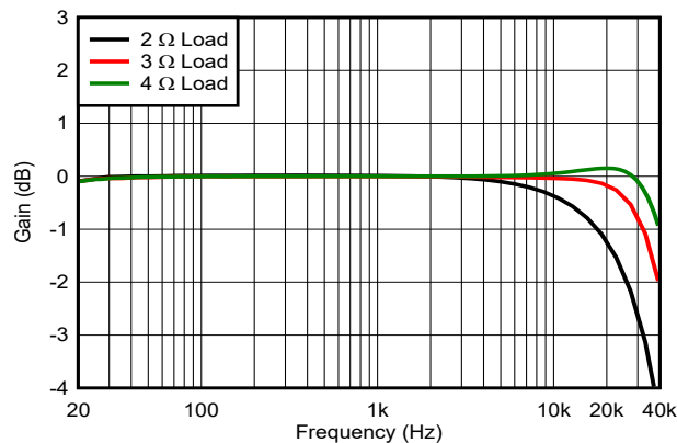
Figure 5-95. Gain vs Frequency
