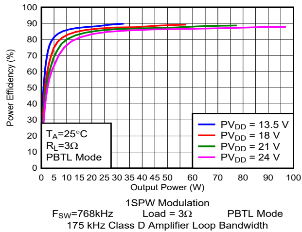
Figure 5-110. Efficiency vs Output Power
