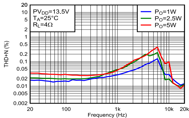
Figure 5-46. THD+N vs Frequency
