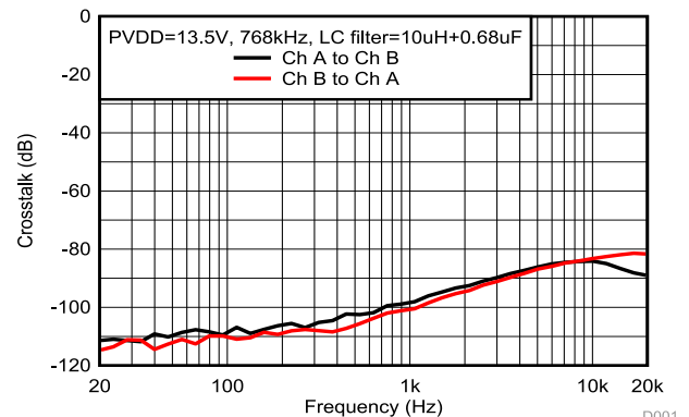
Figure 5-77. Crosstalk
