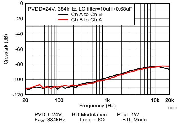
Figure 5-37. Crosstalk
