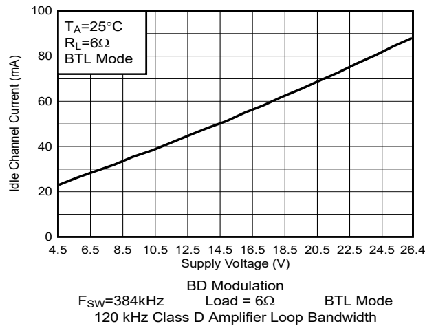
Figure 5-39. PVDD Idle Current vs PVDD Voltage
