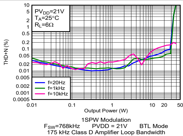
Figure 5-64. THD+N vs Output Power
