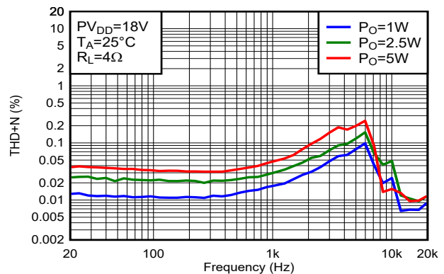
Figure 5-47. THD+N vs Frequency
