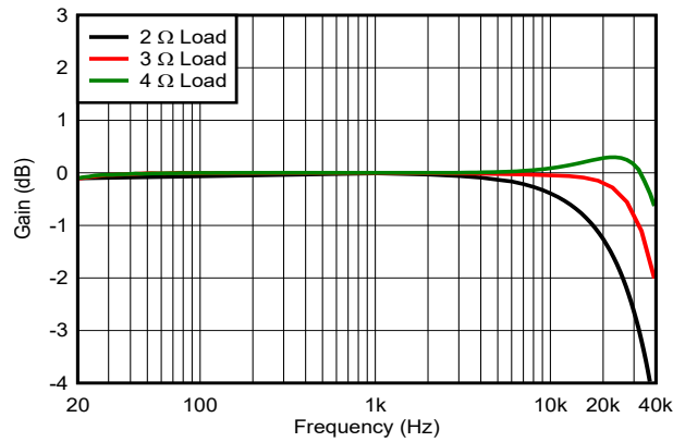
Figure 5-108. Gain vs Frequency
