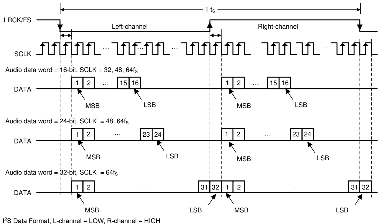
Figure 6-3. I²S Audio Data Format
