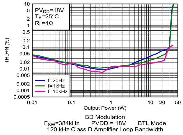
Figure 5-16. THD+N vs Output Power
