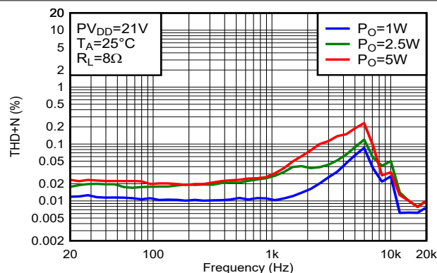
Figure 5-54. THD+N vs Frequency
