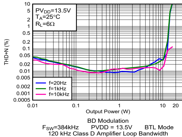
Figure 5-19. THD+N vs Output Power
