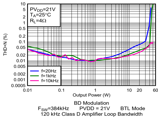
Figure 5-17. THD+N vs Output Power
