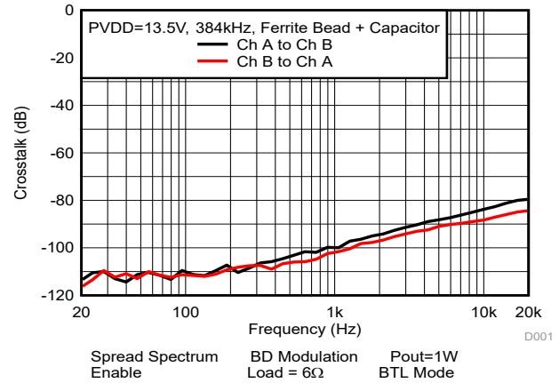
Figure 5-38. Crosstalk
