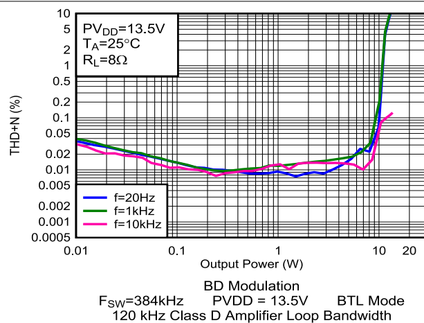
Figure 5-23. THD+N vs Output Power
