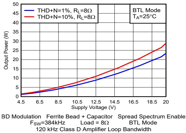
Figure 5-33. Output Power vs Supply Voltage
