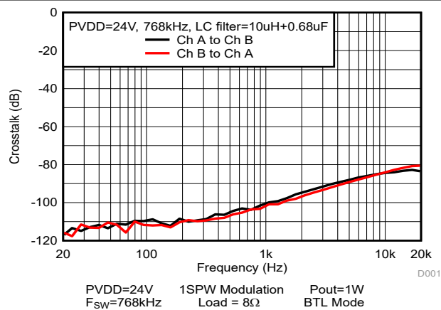
Figure 5-80. Crosstalk
