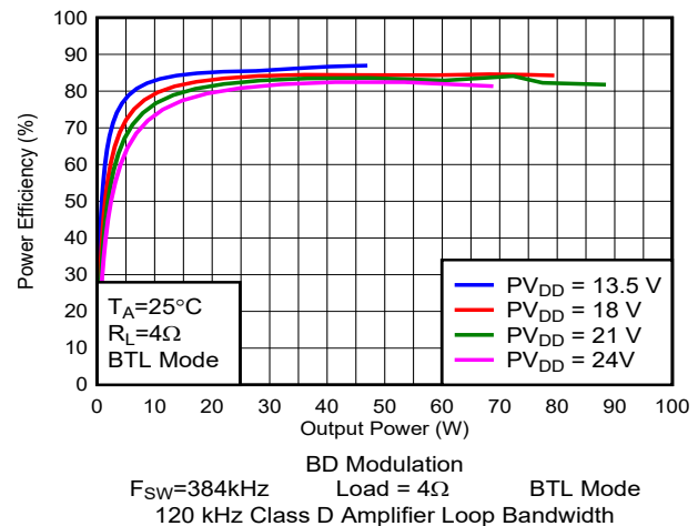
Figure 5-40. Efficiency vs Output Power
