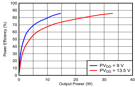
Figure 5-44. Efficiency vs Output Power
