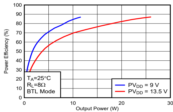
Figure 5-43. Efficiency vs Output Power (with FB)
