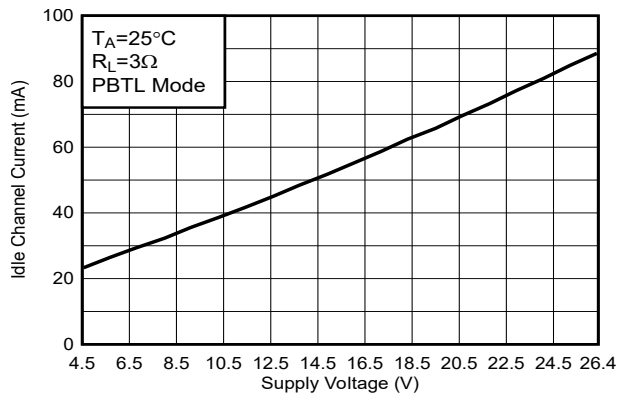
Figure 5-96. PVDD Idle Current vs PVDD voltage
