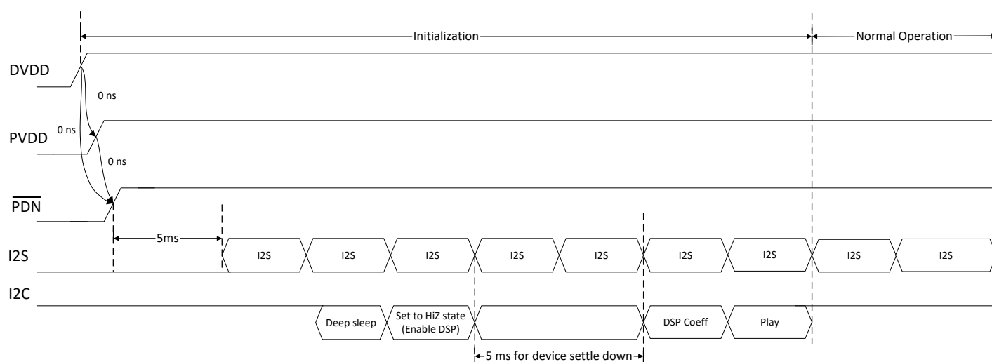
Figure 6-14. Startup sequence
