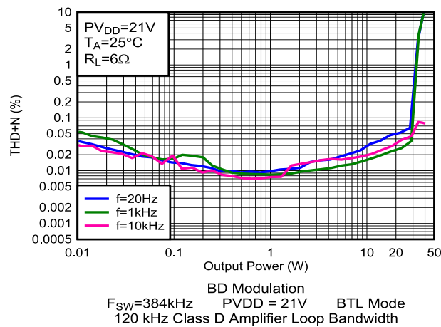
Figure 5-21. THD+N vs Output Power
