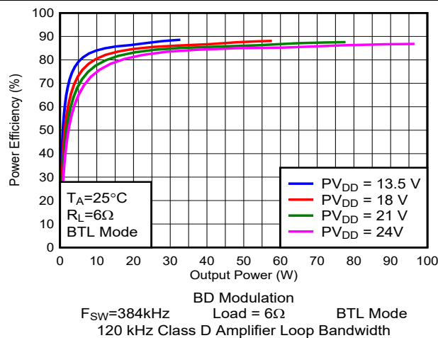
Figure 5-41. Efficiency vs Output Power
