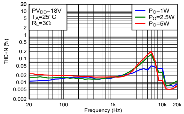
Figure 5-86. THD+N vs Frequency
