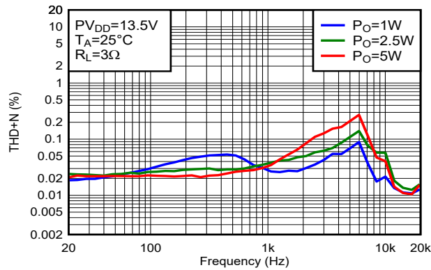
Figure 5-98. THD+N vs Frequency
