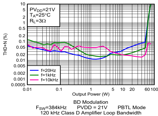
Figure 5-91. THD+N vs Output Power
