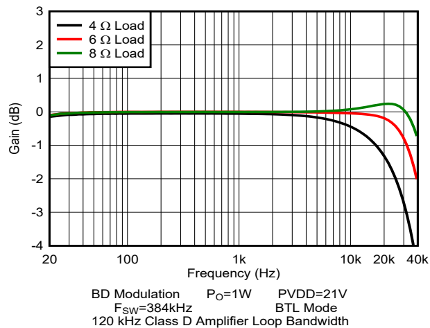
Figure 5-35. Gain vs Frequency
