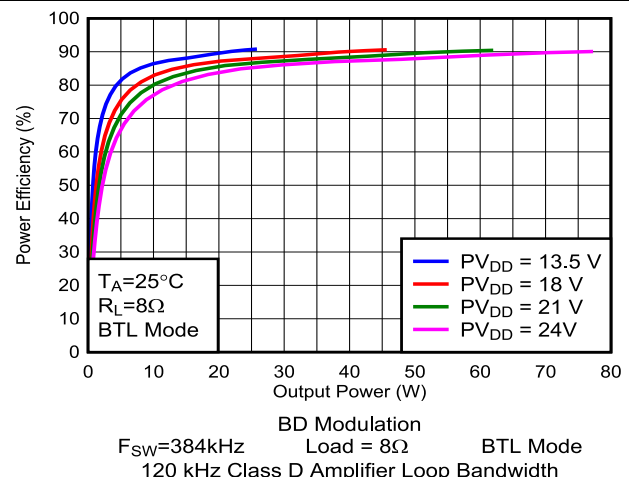
Figure 5-42. Efficiency vs Output Power
