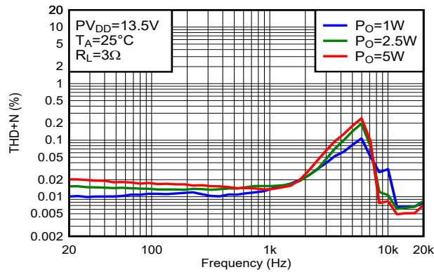
Figure 5-85. THD+N vs Frequency
