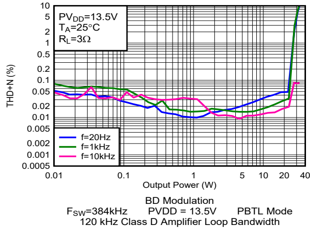
Figure 5-89. THD+N vs Output Power
