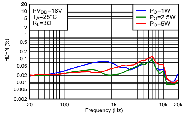
Figure 5-99. THD+N vs Frequency
