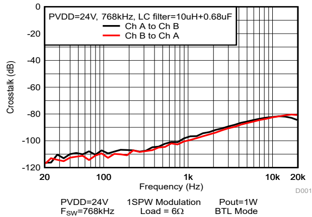
Figure 5-78. Crosstalk
