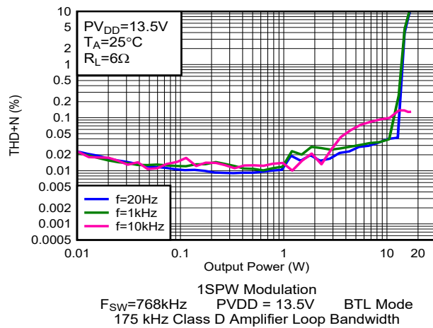
Figure 5-62. THD+N vs Output Power
