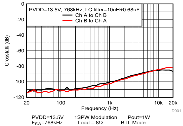
Figure 5-79. Crosstalk
