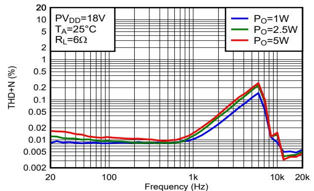
Figure 5-4. THD+N vs Frequency
