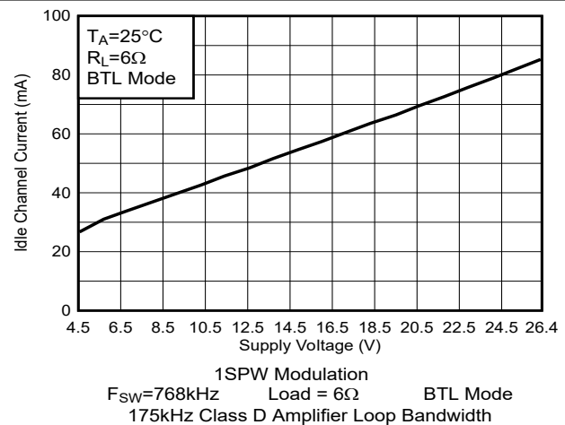
Figure 5-81. PVDD Idle Current vs PVDD Voltage
