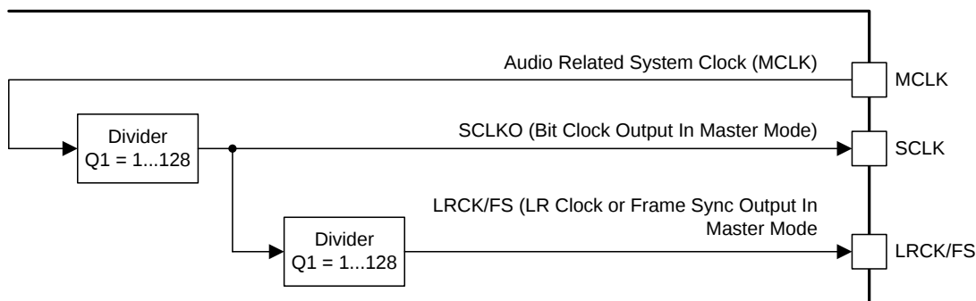
Figure 62. Simplified Clock Tree for MCLK Sourced Master Mode
