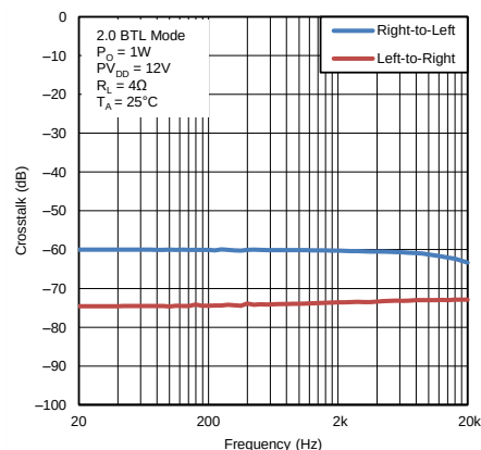
Figure 28. Crosstalk vs Frequency (2.0 BTL Mode)
