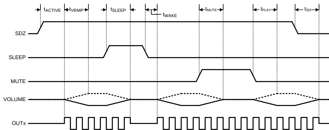
Figure 4. Mode Timing
