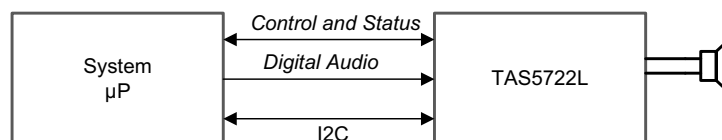
Simplified Schematic
