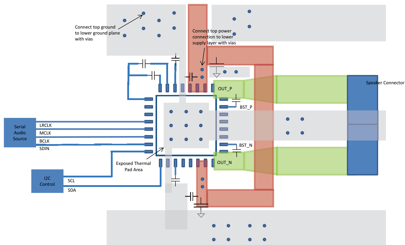
Figure 54. Layout Example
